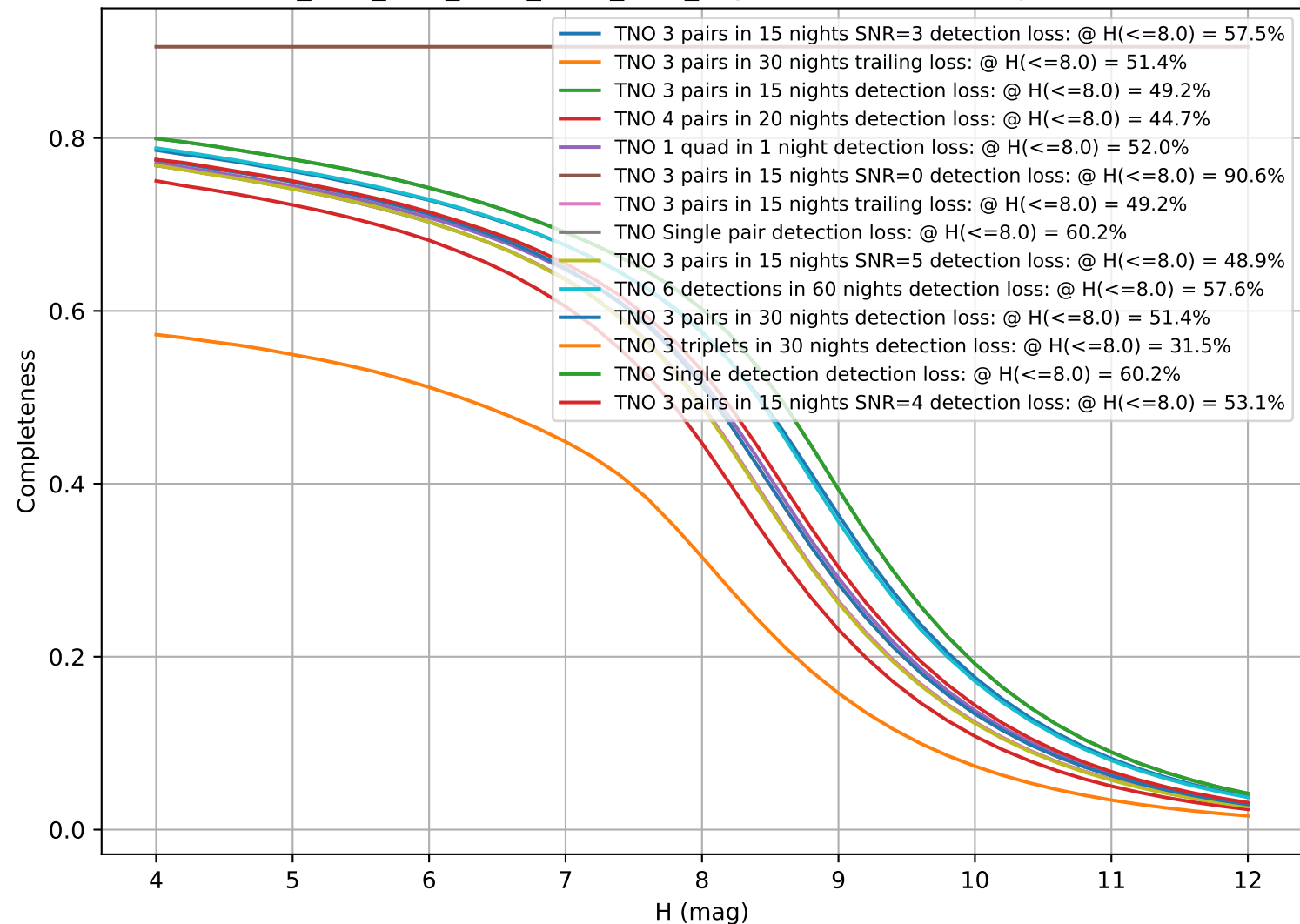
ddf_acor_sf15_lsf20_lsr50_v3.4_10yrs: CumulativeCompleteness
