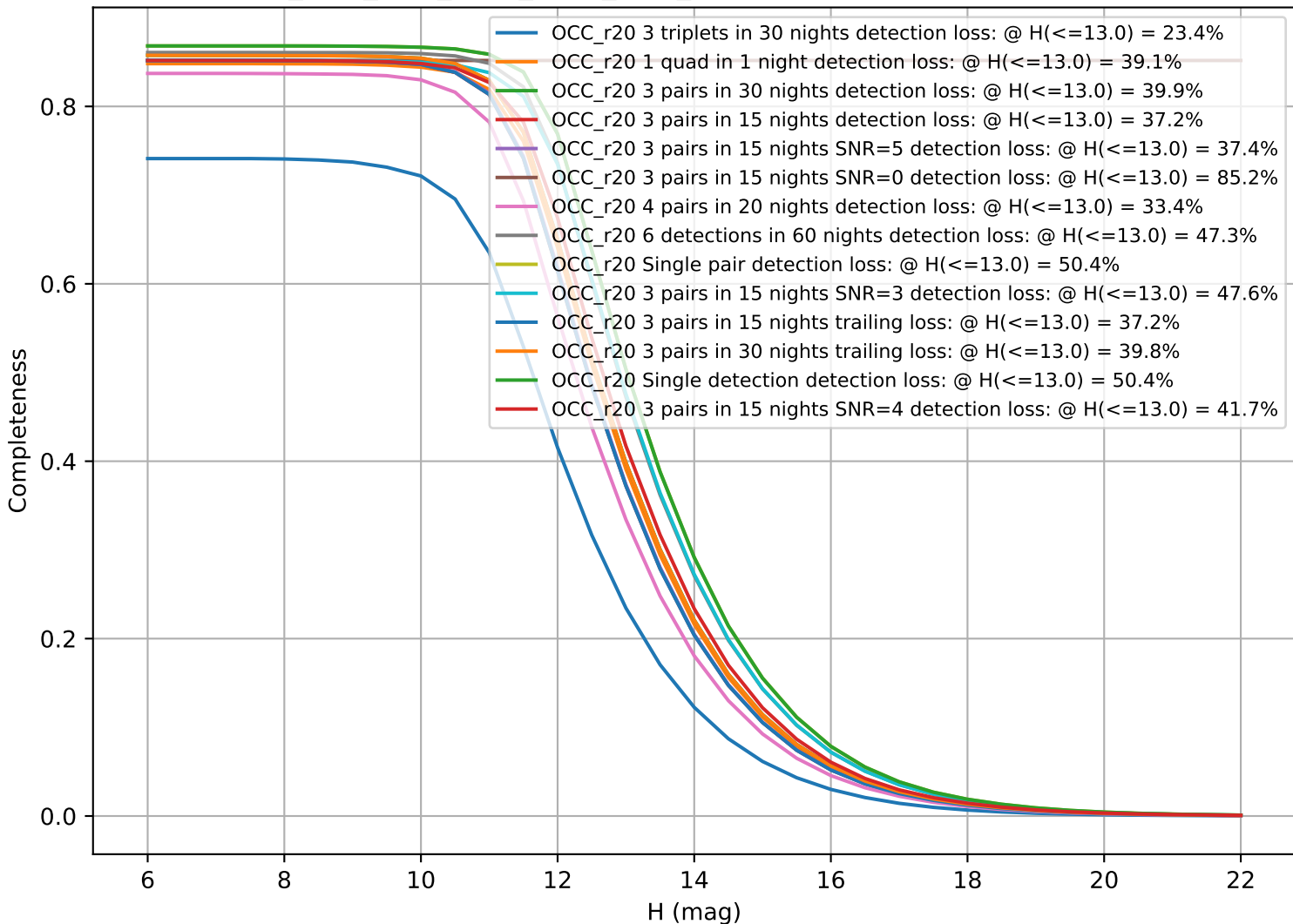
ddf_acor_sf15_lsf20_lsr50_v3.4_10yrs: CumulativeCompleteness
