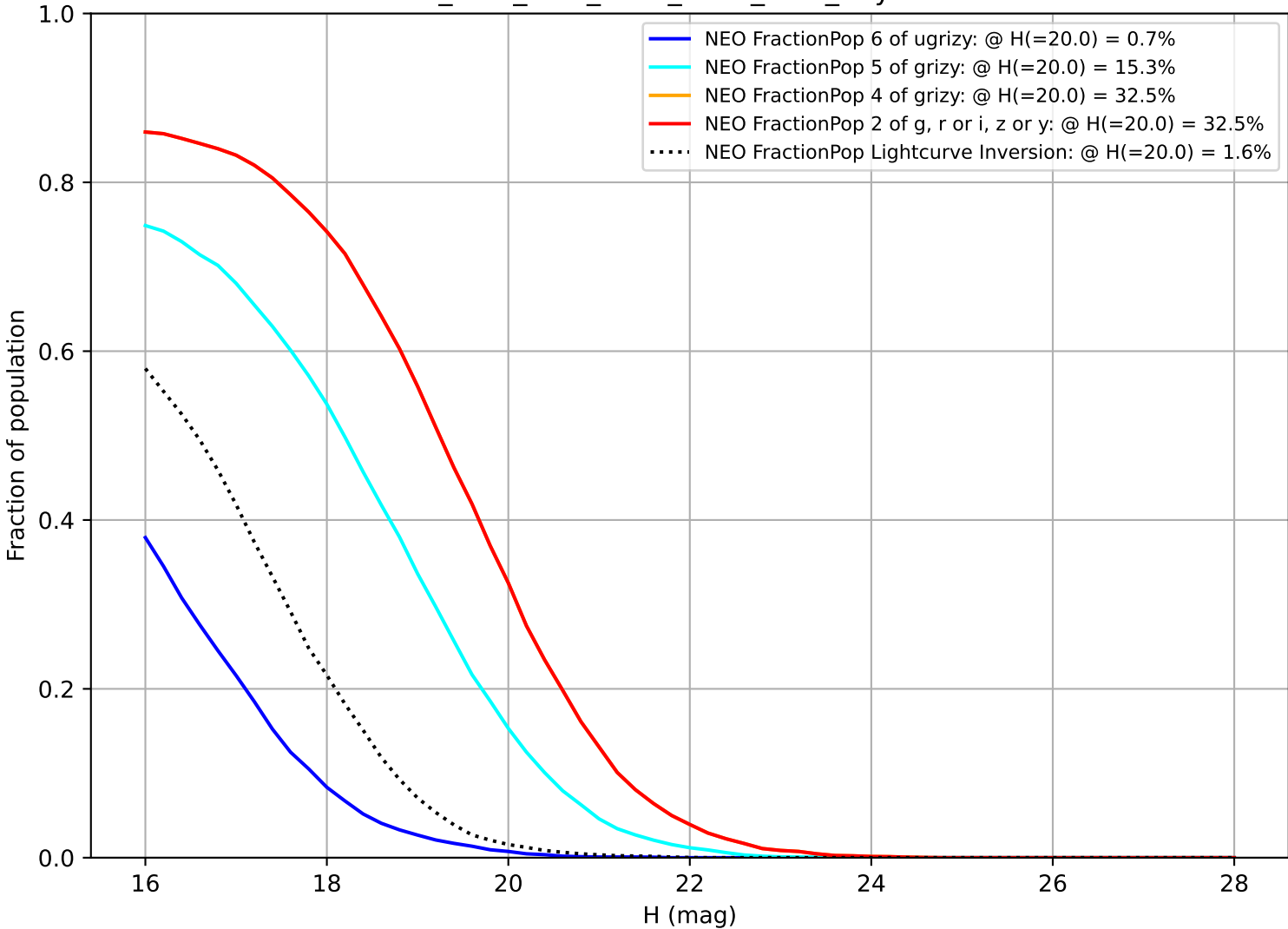
ddf_acor_sf15_lsf20_lsr50_v3.4_10yrs NEO
