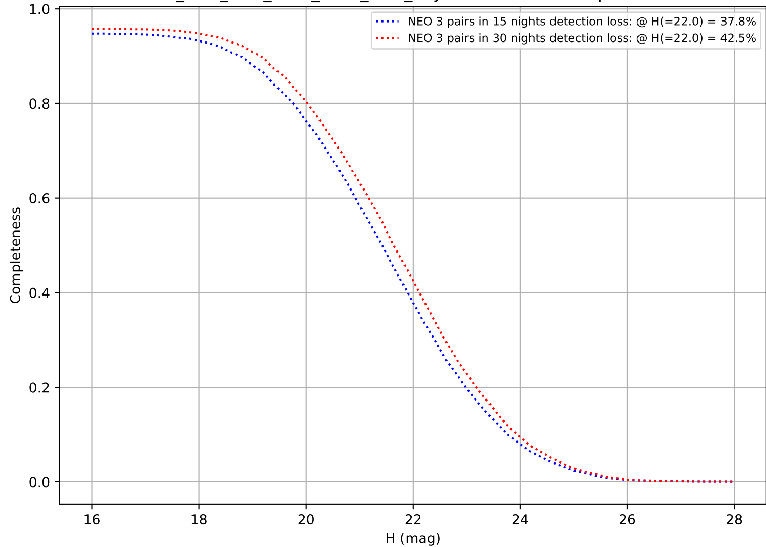
ddf_acor_sf15_lsf20_lsr50_v3.4_10yrs: DifferentialCompleteness
