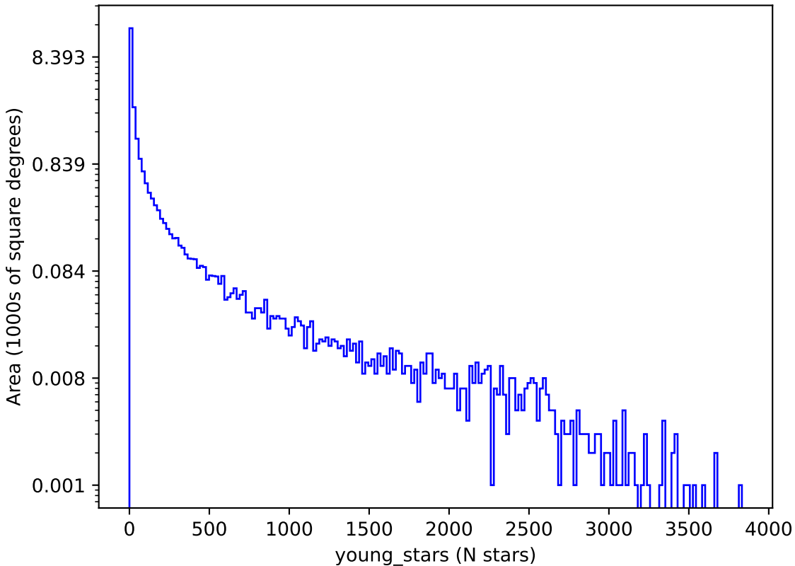
ddf_acor_sf15_lsf20_lsr50_v3.4_10yrs : young_stars
