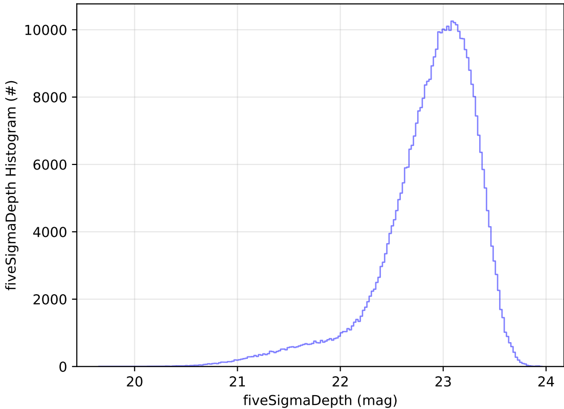
ddf_acor_sf15_lsf20_lsr50_v3.4_10yrs z: fiveSigmaDepth Histogram
