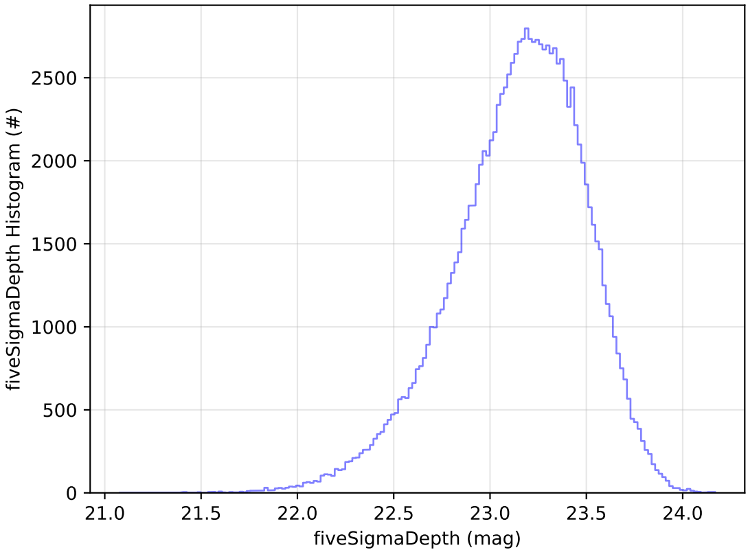
ddf_acor_sf15_lsf20_lsr50_v3.4_10yrs u: fiveSigmaDepth Histogram
