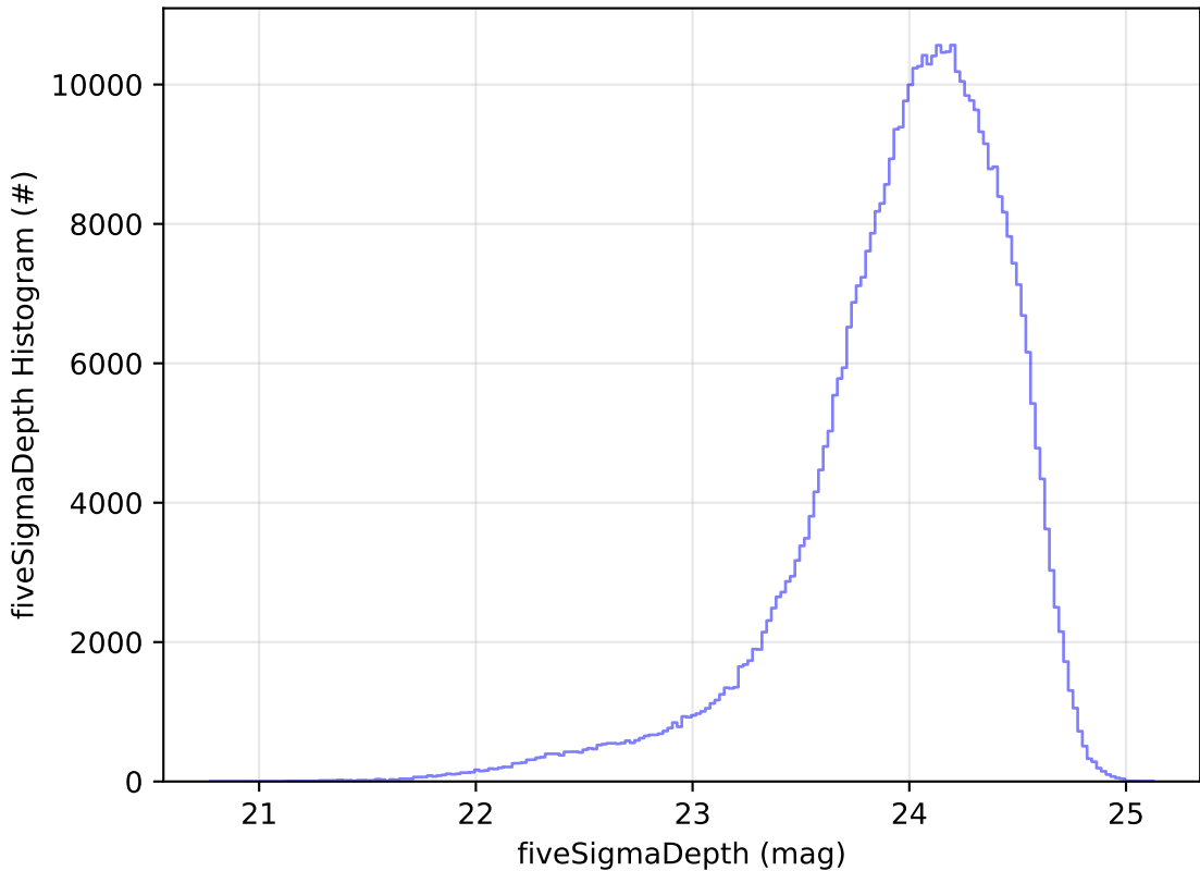
ddf_acor_sf15_lsf20_lsr50_v3.4_10yrs r: fiveSigmaDepth Histogram
