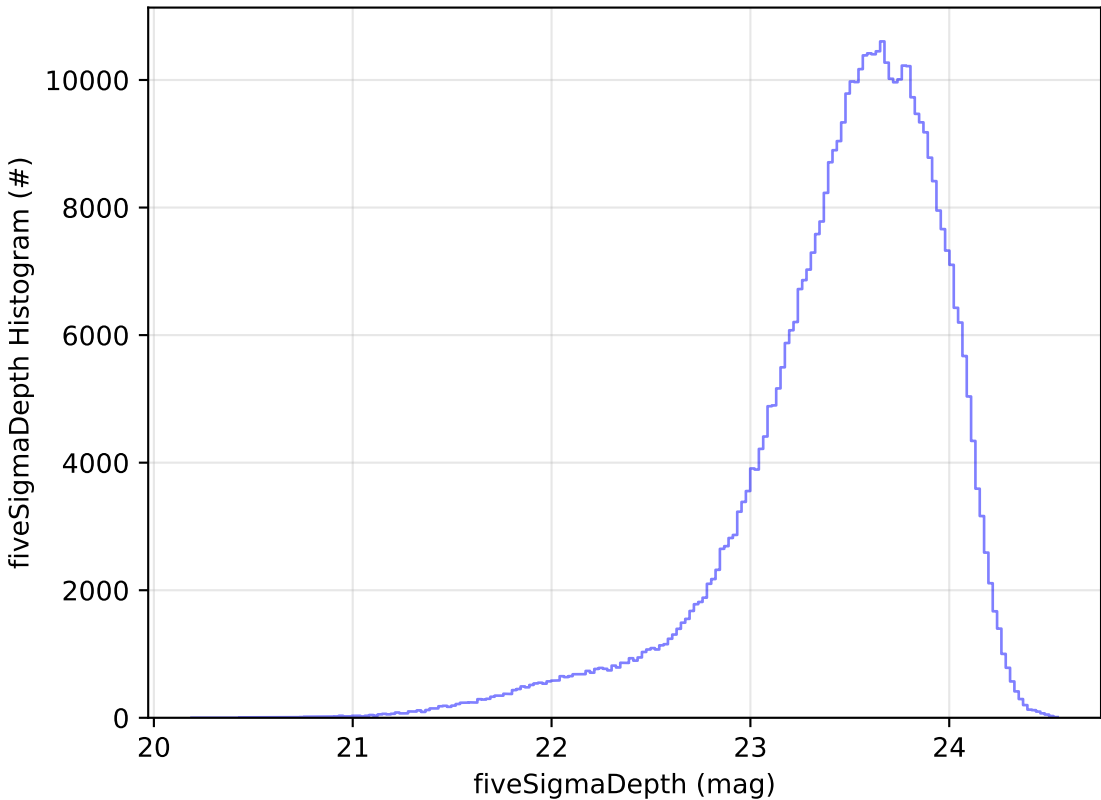
ddf_acor_sf15_lsf20_lsr50_v3.4_10yrs i: fiveSigmaDepth Histogram
