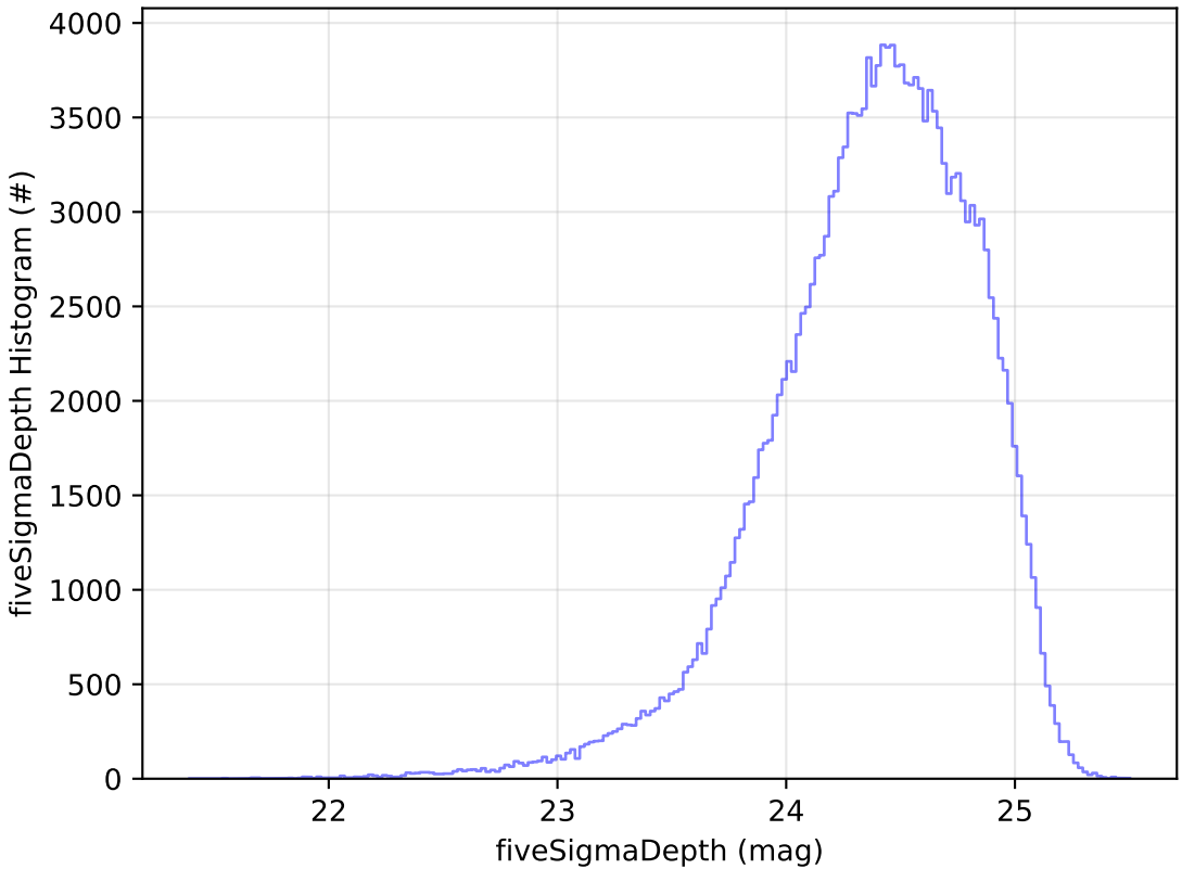
ddf_acor_sf15_lsf20_lsr50_v3.4_10yrs g: fiveSigmaDepth Histogram
