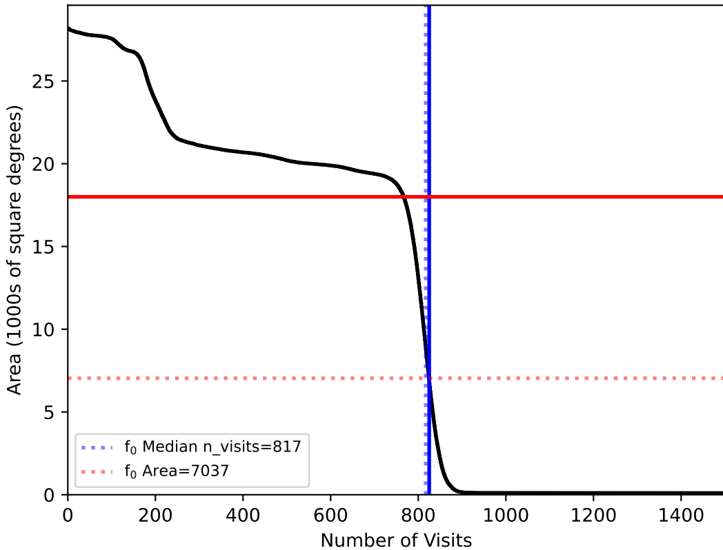
ddf_acor_sf15_lsf20_lsr50_v3.4_10yrs : fO
