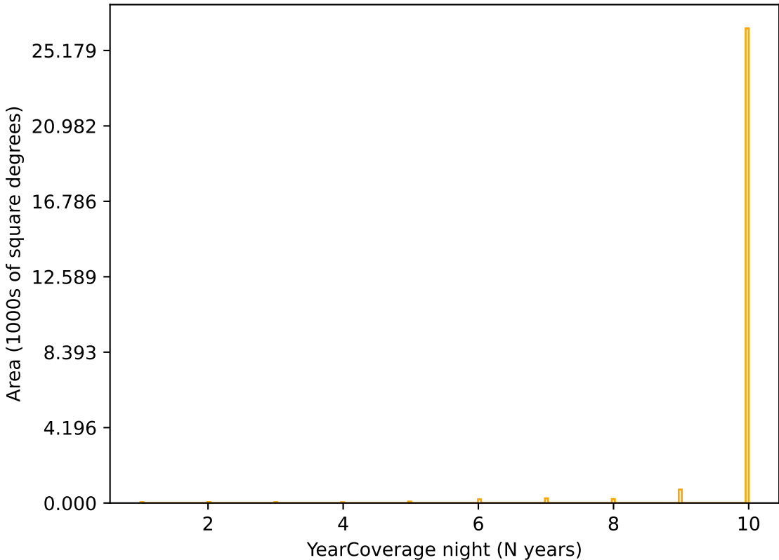
ddf_acor_sf15_lsf20_lsr50_v3.4_10yrs r band: YearCoverage night
