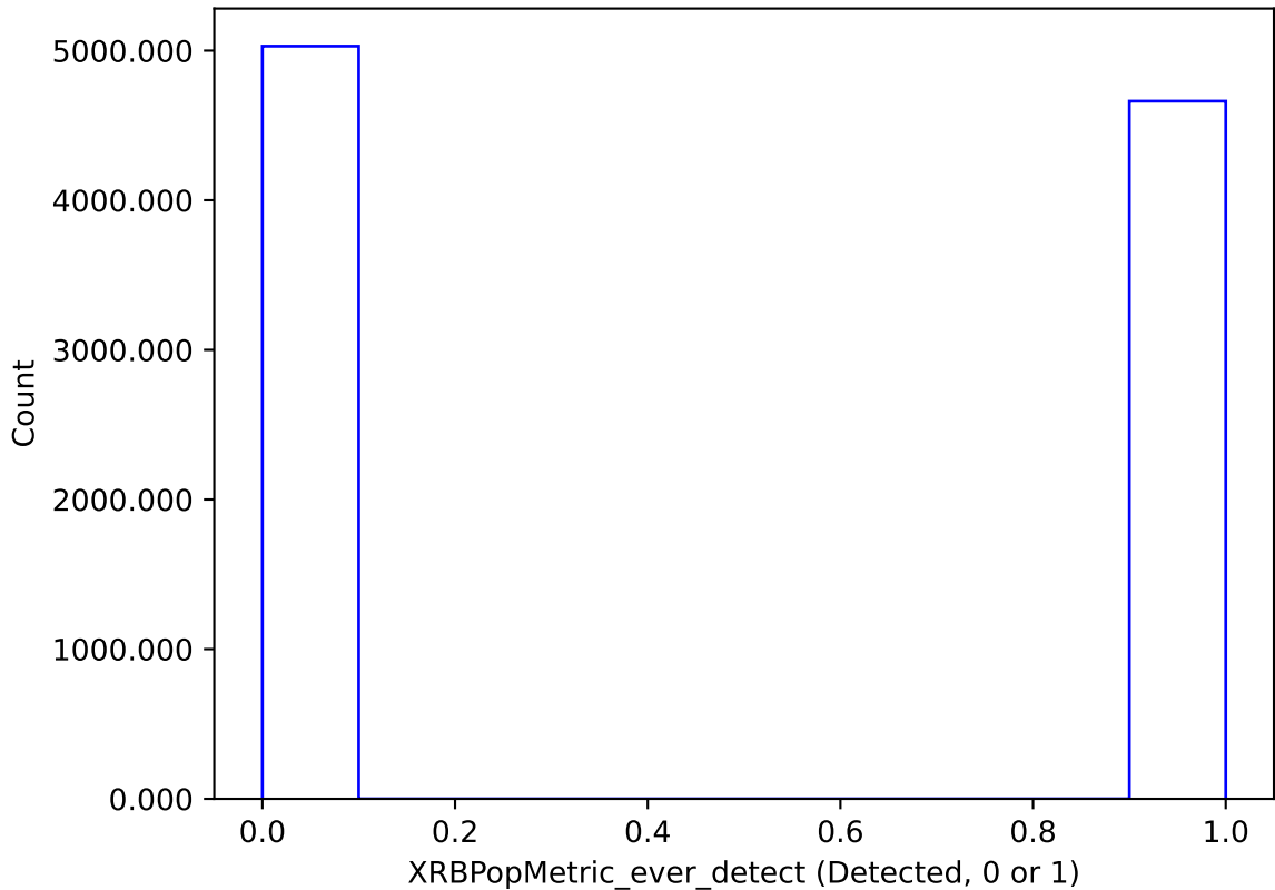
ddf_acor_sf15_lsf20_lsr50_v3.4_10yrs : XRBPoMetric_ever_detect
