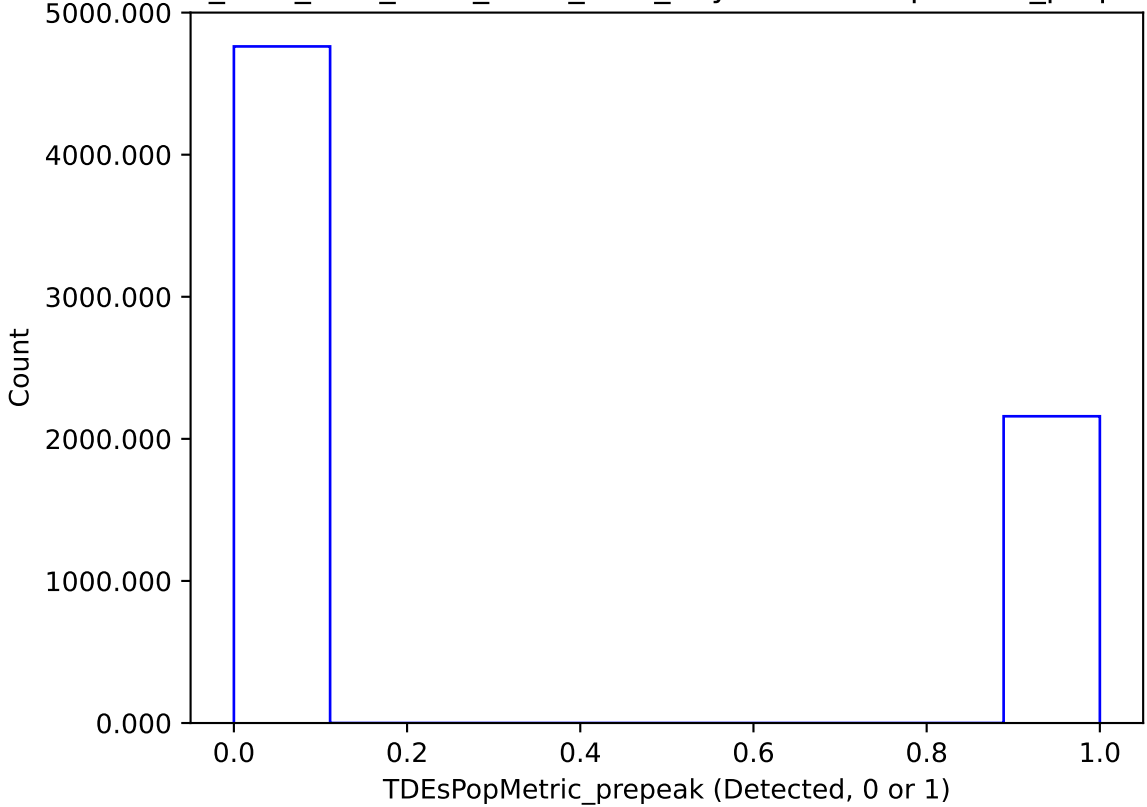
ddf_acor_sf15_lsf20_lsr50_v3.4_10yrs : TDEsPopMetric_prepeak
