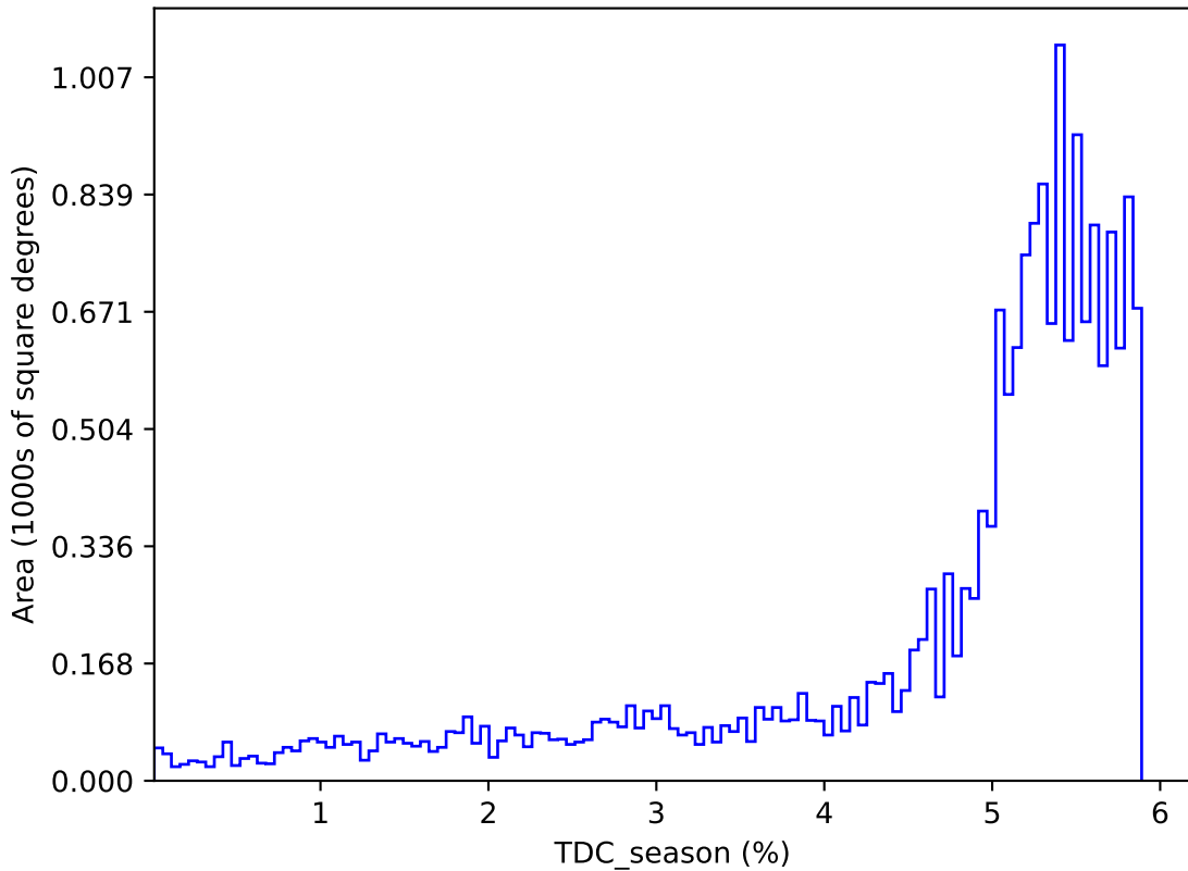
ddf_acor_sf15_lsf20_lsr50_v3.4_10yrs : TDC_season
