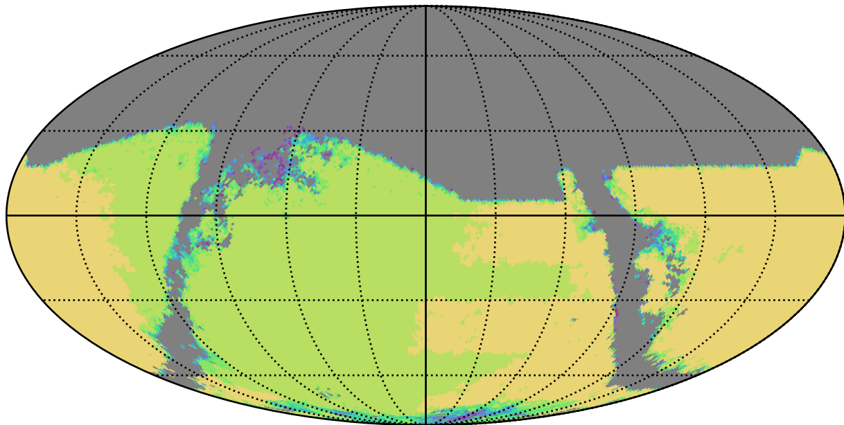
ddf_acor_sf15_lsf20_lsr50_v3.4_10yrs : TDC_campaign
