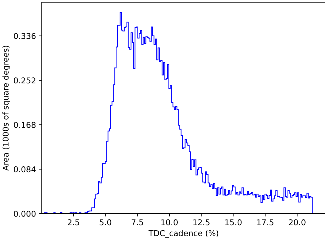
ddf_acor_sf15_ls20_lsr50_v3.4_10yrs : TDC_cadence
