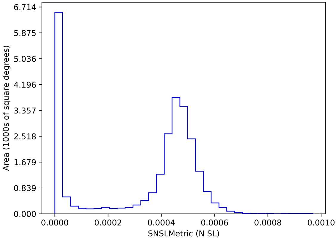
ddf_acor_sf15_ls20_lsr50_v3.4_10yrs : SNSLMetric
