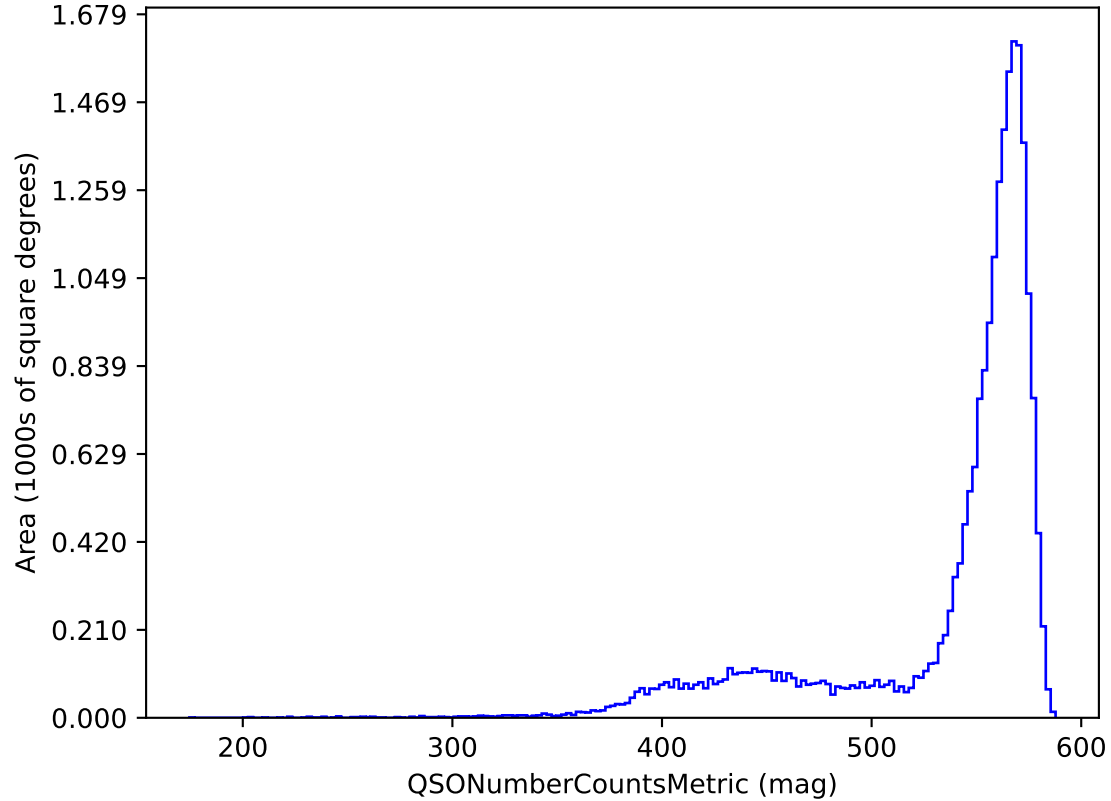
ddf_acor_sf15_lsf20_lsr50_v3.4_10yrs y band and non-DD: QSONumberCountsMetric
