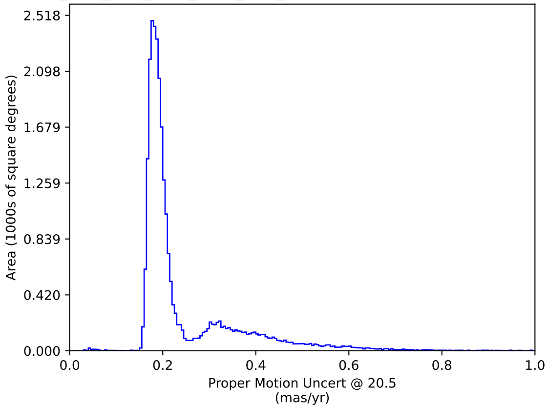
ddf_acor_sf15_lsf20_lsr50_v3.4_10yrs : Proper Motion Uncert @ 20.5
