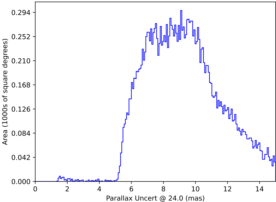
ddf_acor_sf15_lsf20_lsr50_v3.4_10yrs : Parallax Uncert @ 24.0
