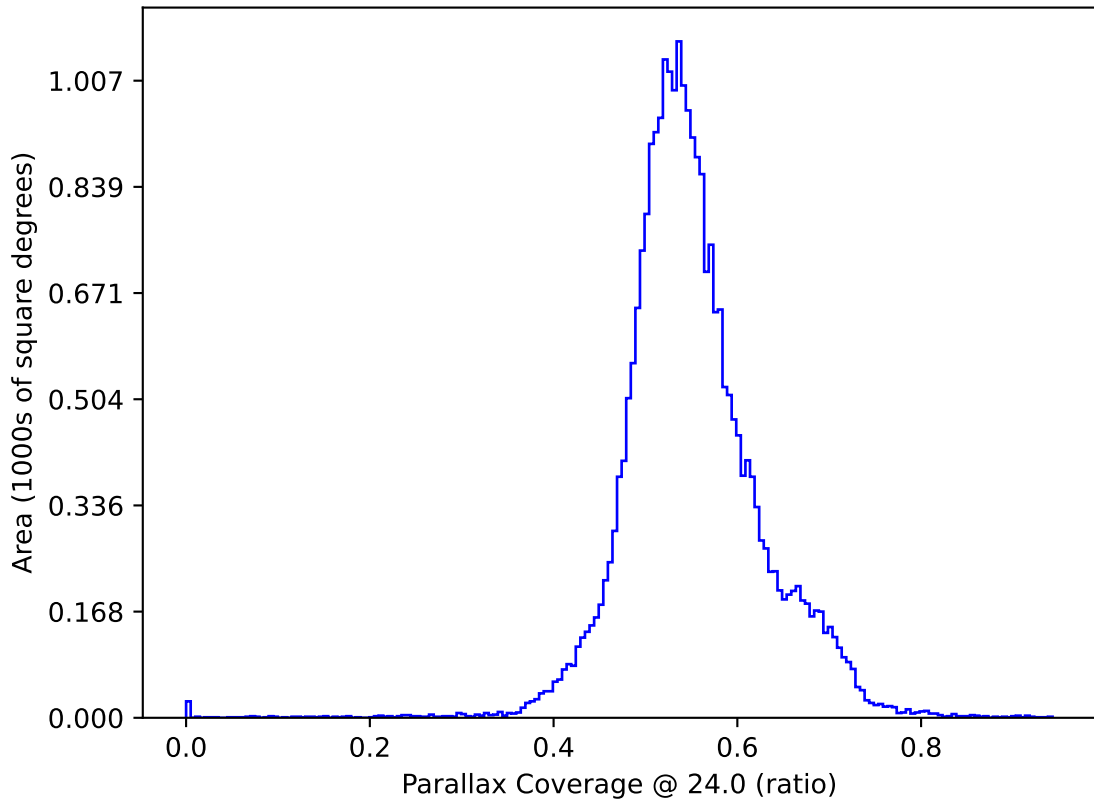
ddf_acor_sf15_lsf20_lsr50_v3.4_10yrs : Parallax Coverage @ 24.0
