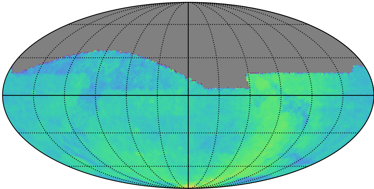
ddf_acor_sf15_lsf20_lsr50_v3.4_10yrs : Parallax Coverage @ 22.4
