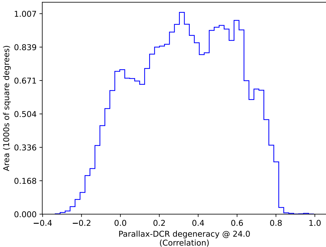
ddf_acor_sf15_ls20_lsr50_v3.4_10yrs : Parallax-DCR degeneracy @ 24.0
