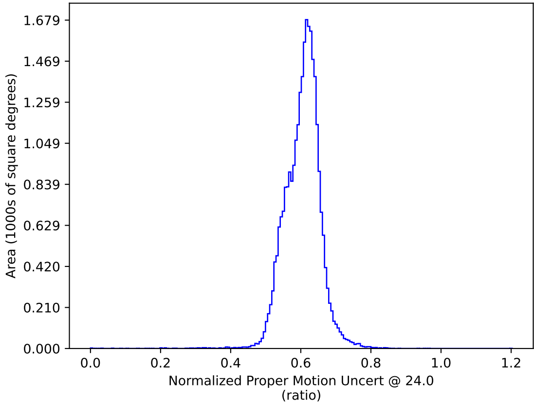
ddf_acor_sf15_lsf20_lsr50_v3.4_10yrs : Normalized Proper Motion Uncert @ 24.0
