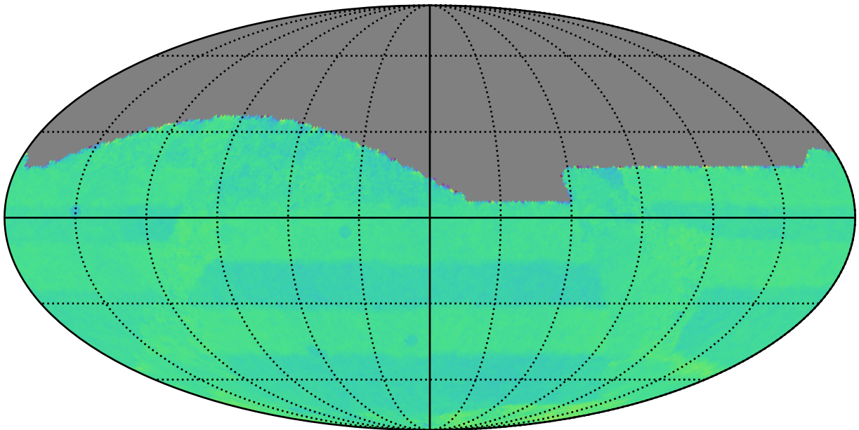
ddf_acor_sf15_lsf20_lsr50_v3.4_10yrs : Normalized Proper Motion Uncert @ 20.5
