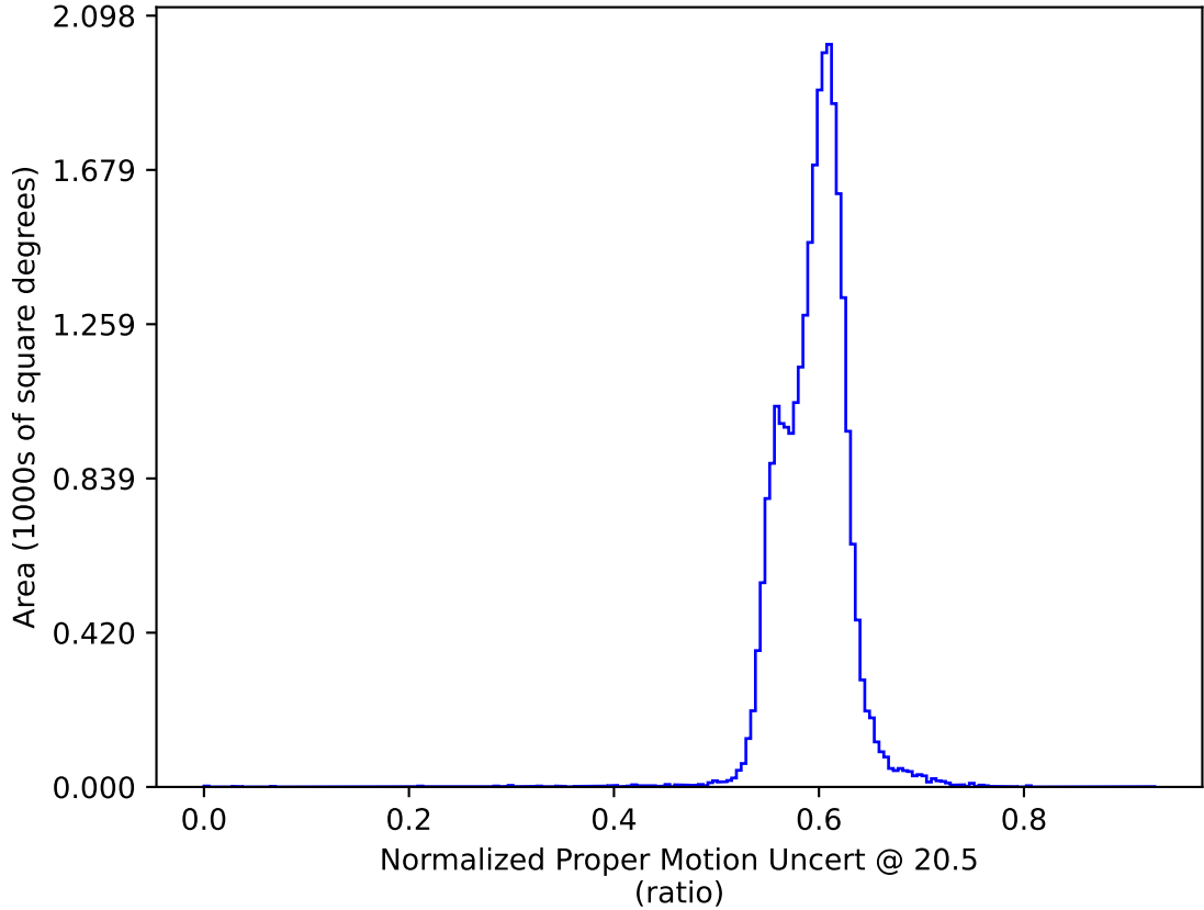
ddf_acor_sf15_lsf20_lsr50_v3.4_10yrs : Normalized Proper Motion Uncert @ 20.5
