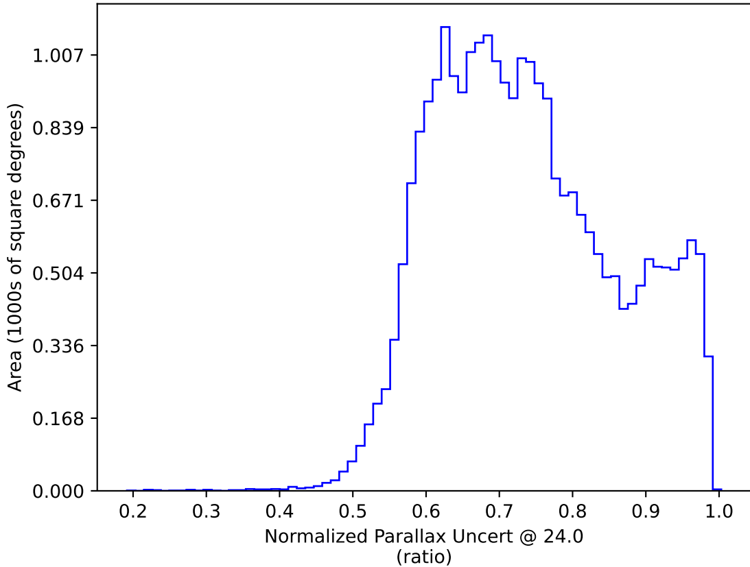
ddf_acor_sf15_lsf20_lsr50_v3.4_10yrs : Normalized Parallax Uncert @ 24.0
