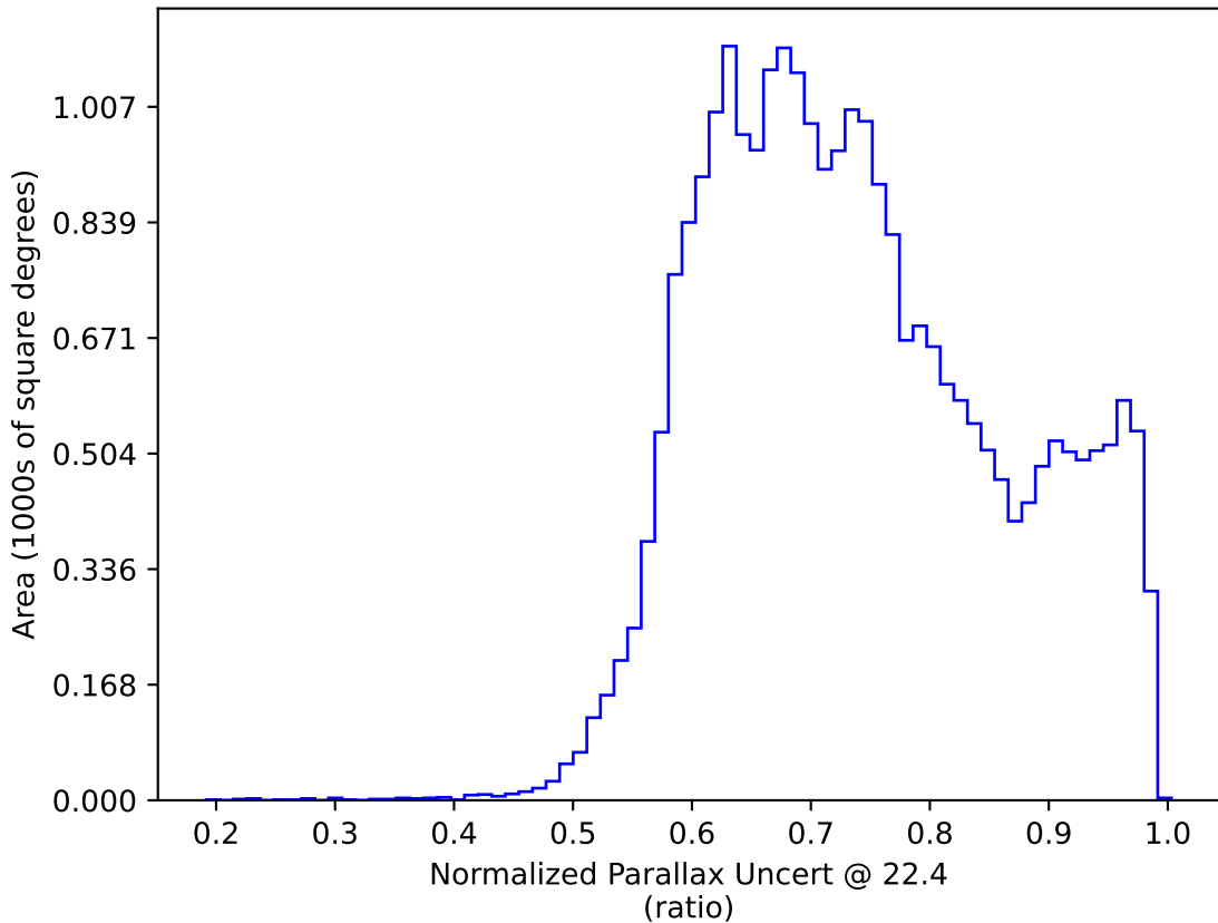
ddf_acor_sf15_lsf20_lsr50_v3.4_10yrs : Normalized Parallax Uncert @ 22.4
