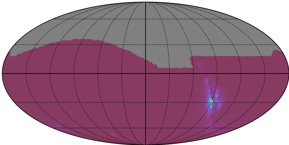
ddf_acor_sf15_lsf20_lsr50_v3.4_10yrs : NlcPoints
