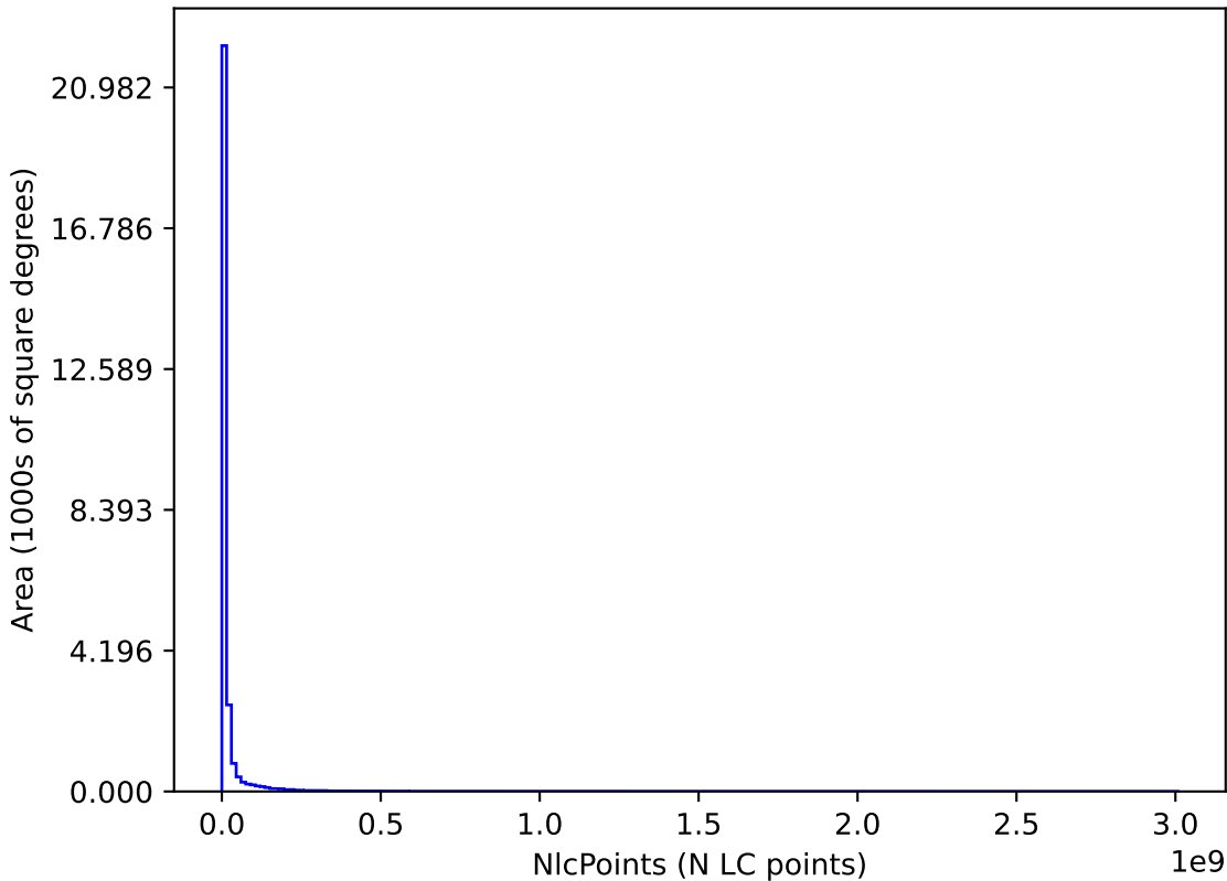
ddf_acor_sf15_lsf20_lsr50_v3.4_10yrs : NlcPoints
