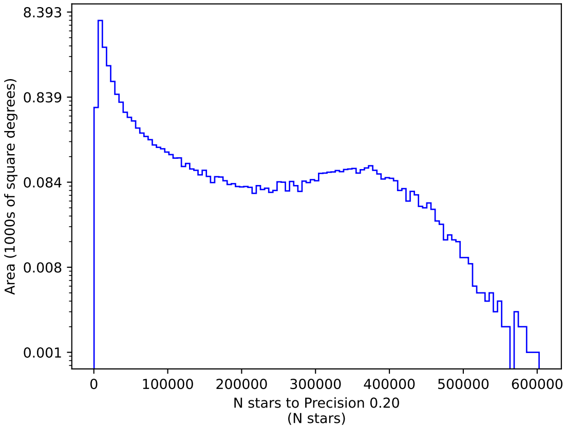
ddf_acor_sf15_lsf20_lsr50_v3.4_10yrs y: N stars to Precision 0.20
