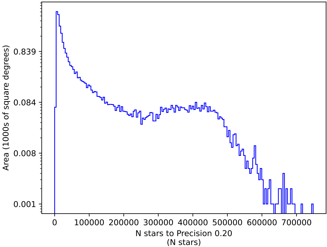
ddf_acor_sf15_lsf20_lsr50_v3.4_10yrs r: N stars to Precision 0.20
