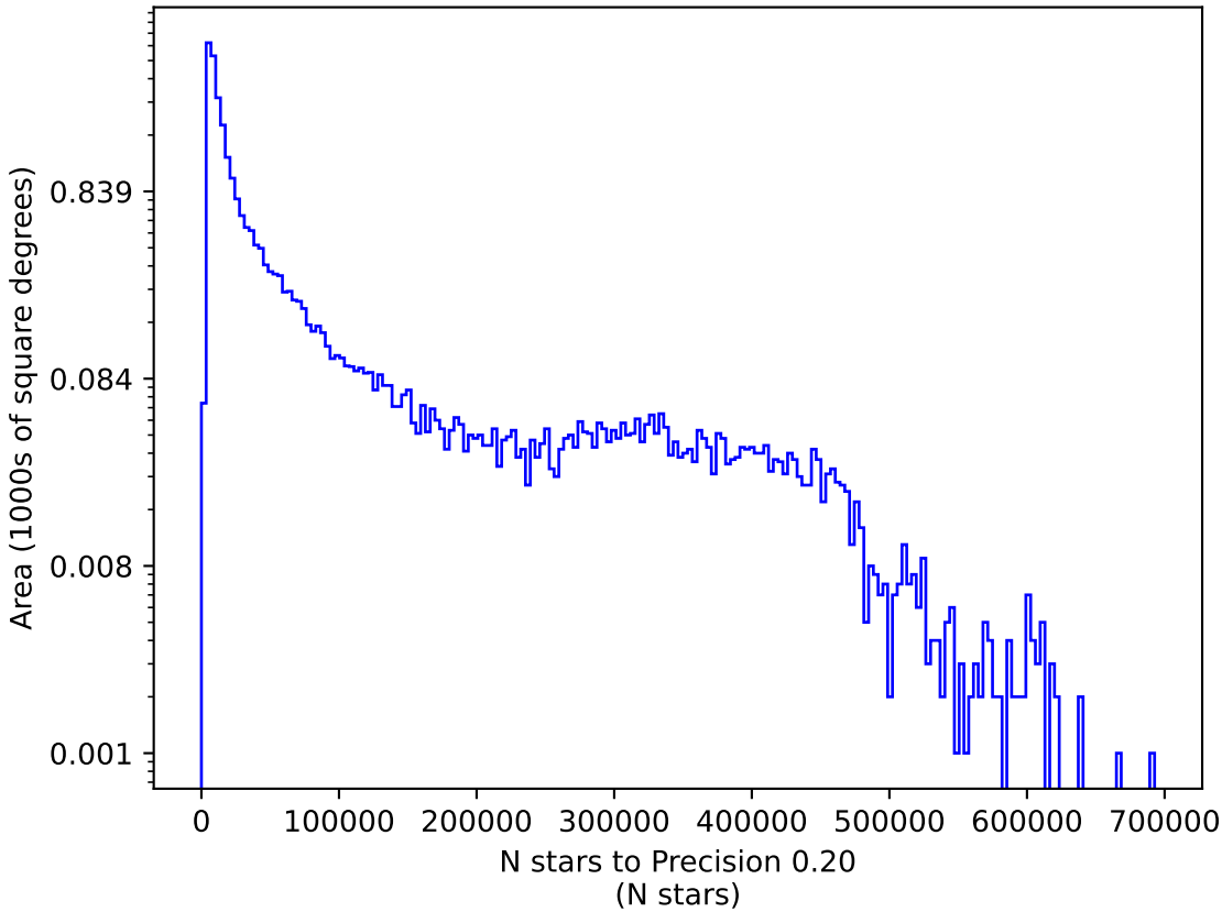
ddf_acor_sf15_lsf20_lsr50_v3.4_10yrs g: N stars to Precision 0.20
