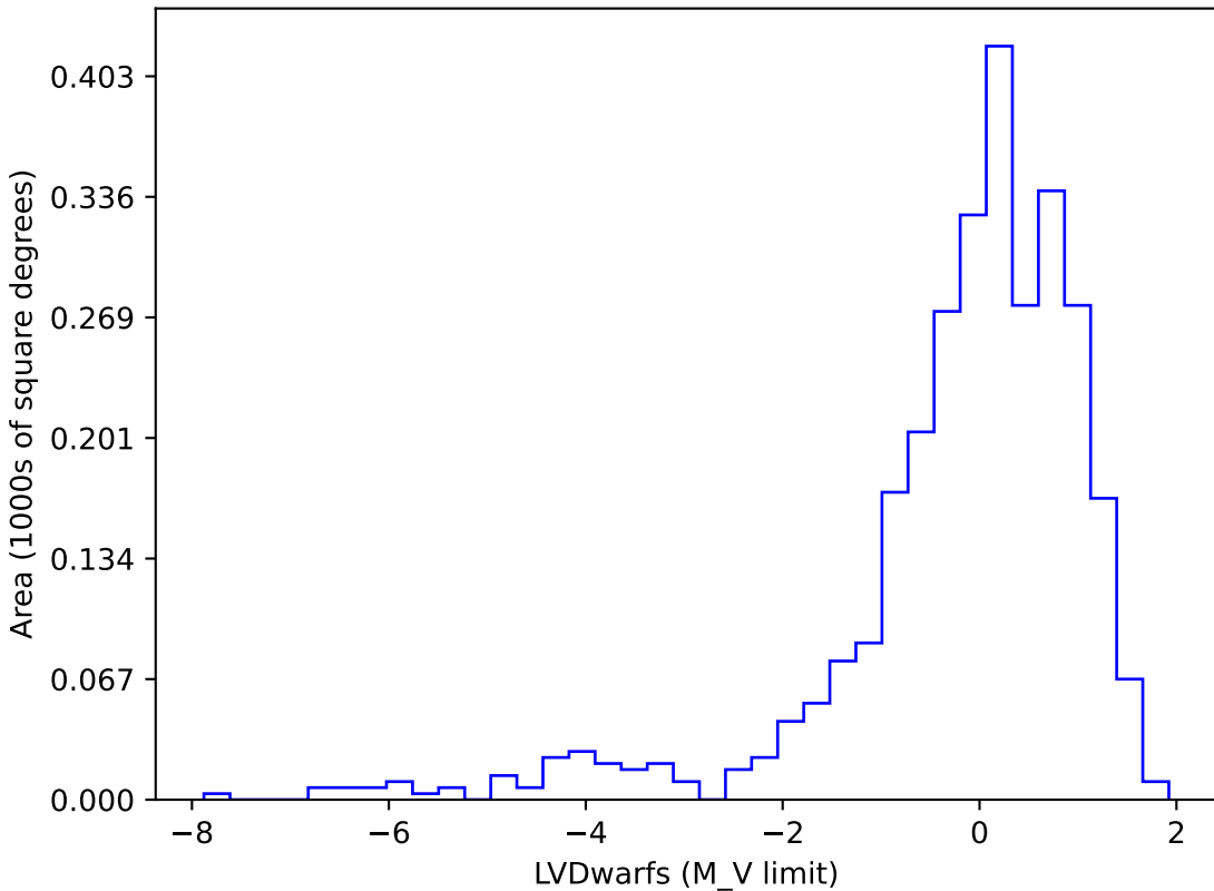
ddf_acor_sf15_lsf20_lsr50_v3.4_10yrs gi SCP: LVDwarfs
