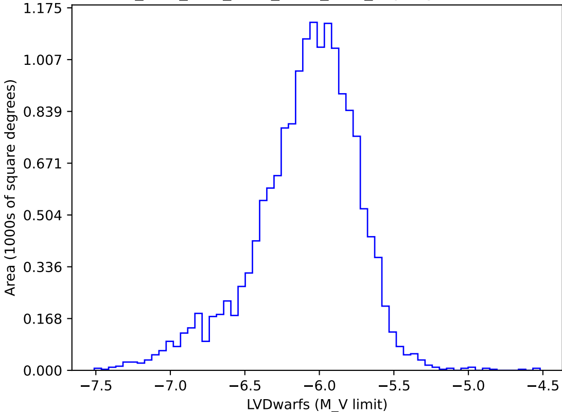
ddf_acor_sf15_lsf20_lsr50_v3.4_10yrs gi: LVDwarfs
