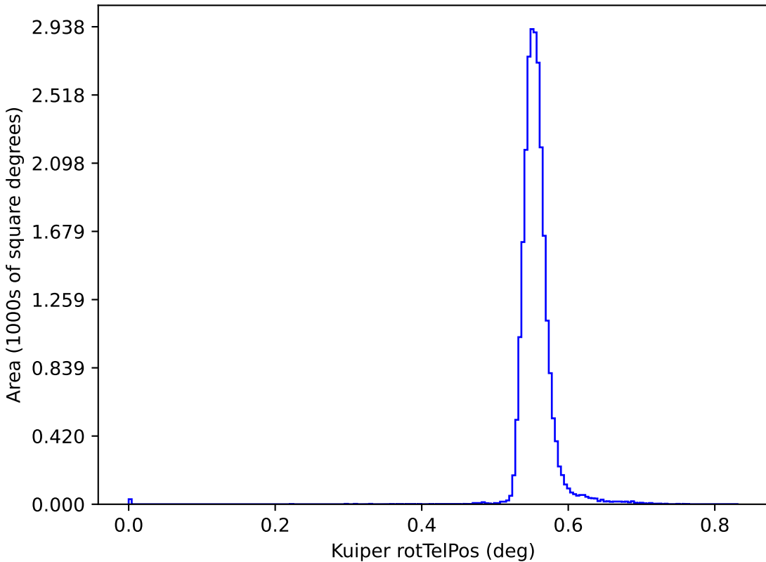
ddf_acor_sf15_ls20_lsr50_v3.4_10yrs y: Kuiper rotTelPos
