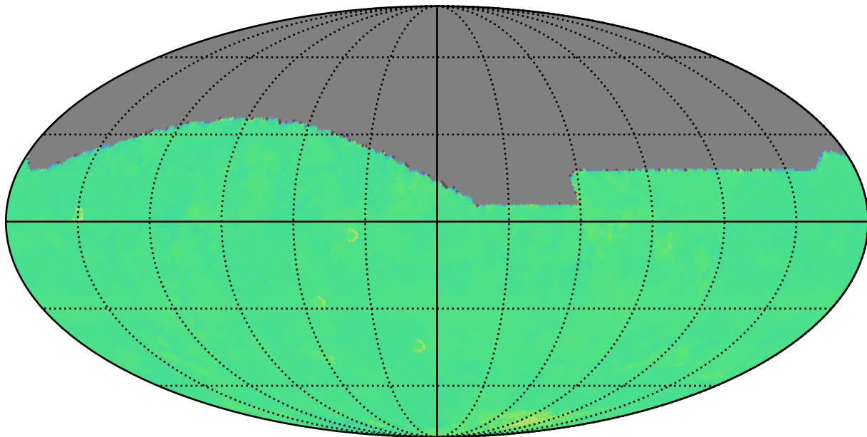
ddf_acor_sf15_lsf20_lsr50_v3.4_10yrs r: Kuiper rotTelPos
