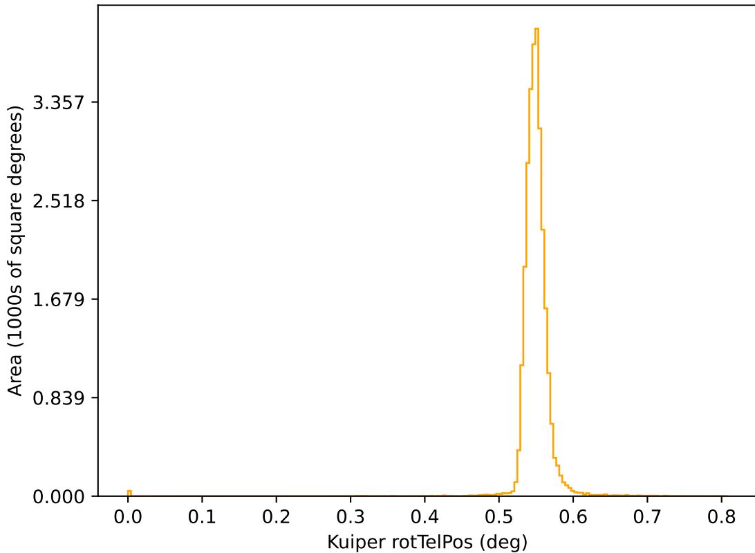
ddf_acor_sf15_lsf20_lsr50_v3.4_10yrs r: Kuiper rotTelPos
