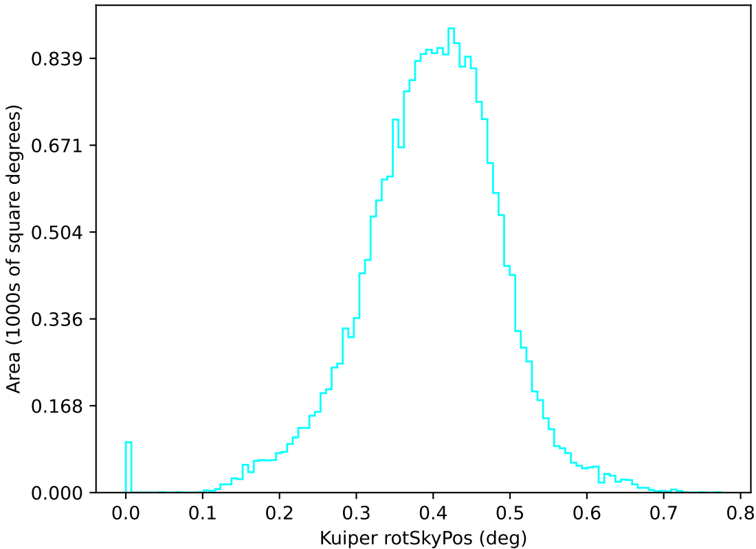
ddf_acor_sf15_lsf20_lsr50_v3.4_10yrs u: Kuiper rotSkyPos
