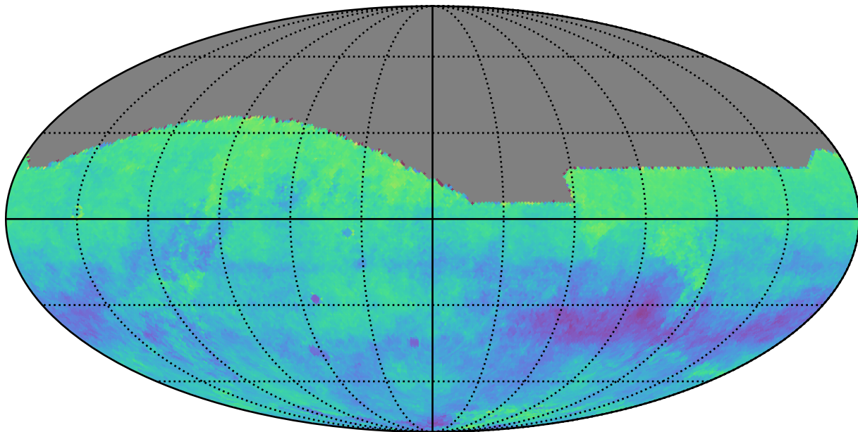
ddf_acor_sf15_lsf20_lsr50_v3.4_10yrs r: Kuiper rotSkyPos
