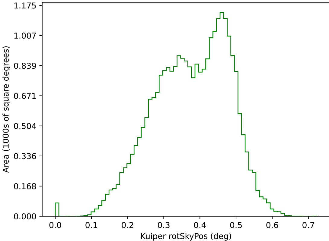
ddf_acor_sf15_lsf20_lsr50_v3.4_10yrs g: Kuiper rotSkyPos
