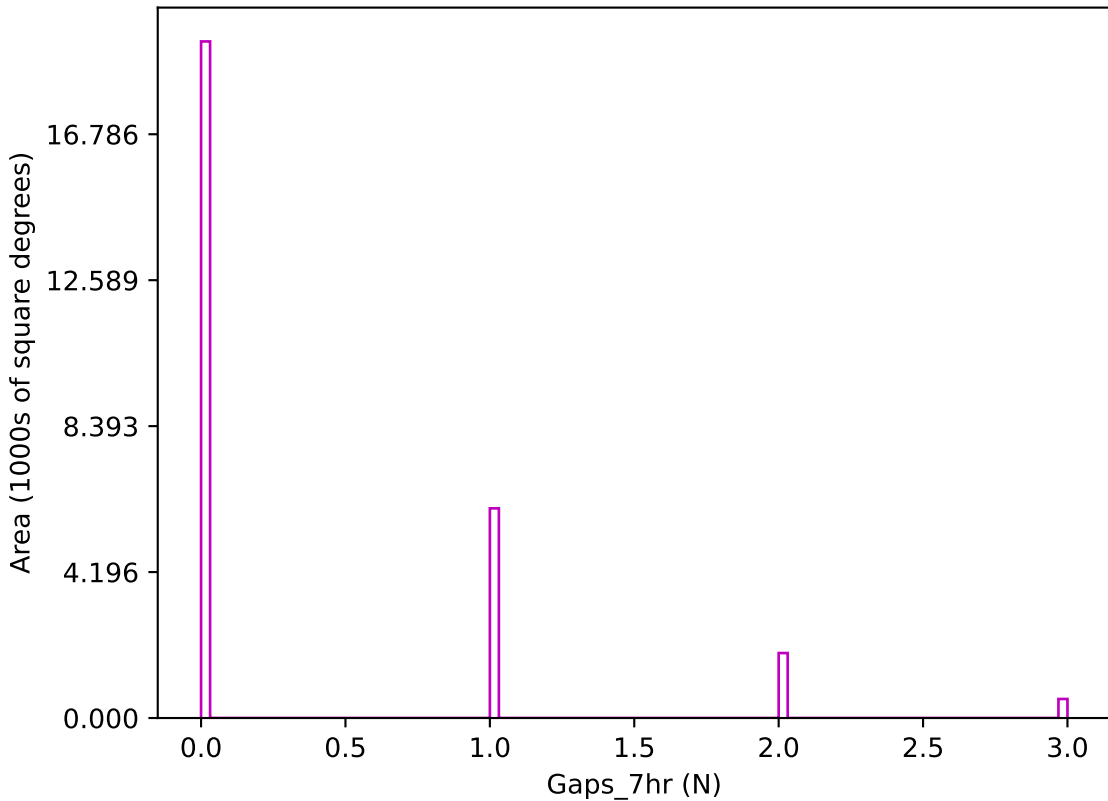
ddf_acor_sf15_lsf20_lsr50_v3.4_10yrs z band: Gaps_7hr
