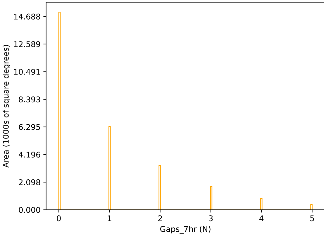
ddf_acor_sf15_lsf20_lsr50_v3.4_10yrs r band: Gaps_7hr
