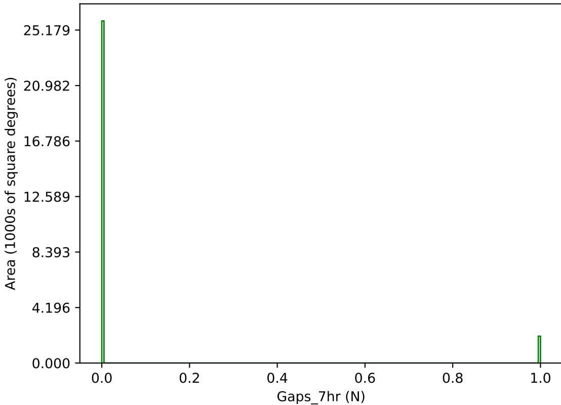
ddf_acor_sf15_lsf20_lsr50_v3.4_10yrs g band: Gaps_7hr
