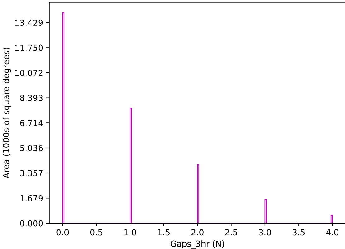
ddf_acor_sf15_lsf20_lsr50_v3.4_10yrs z band: Gaps_3hr
