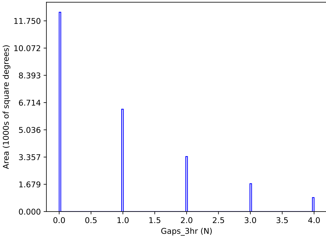
ddf_acor_sf15_lsf20_lsr50_v3.4_10yrs y band: Gaps_3hr
