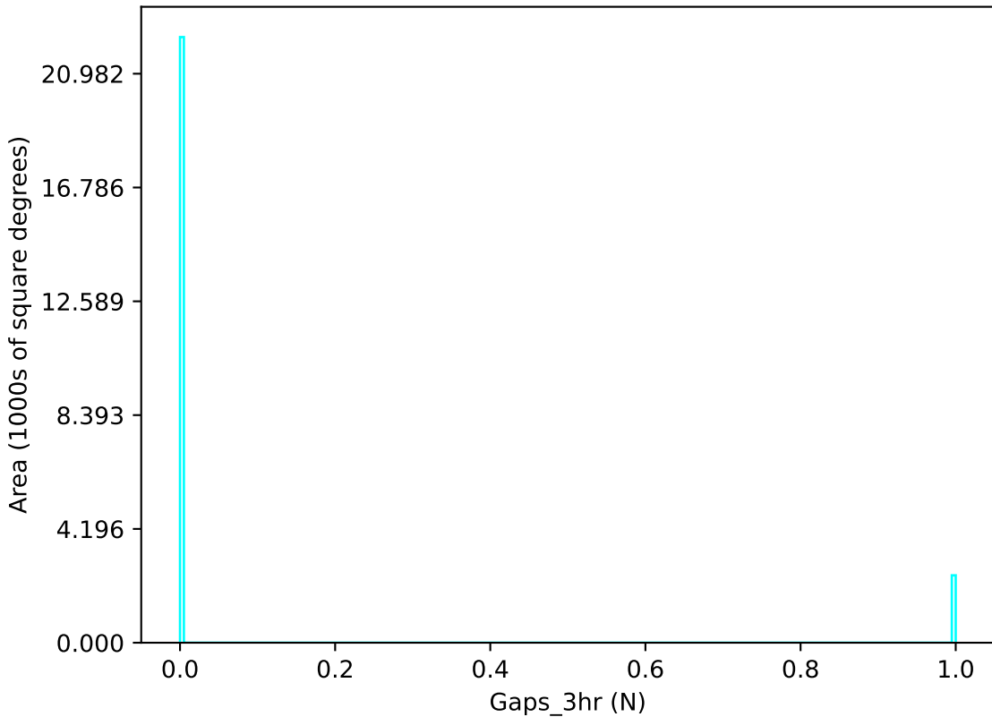
ddf_acor_sf15_lsf20_lsr50_v3.4_10yrs u band: Gaps_3hr
