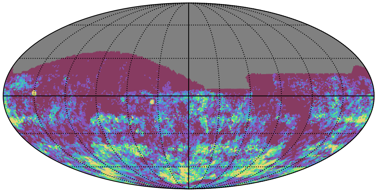
ddf_acor_sf15_lsf20_lsr50_v3.4_10yrs r band: Gaps_3hr
