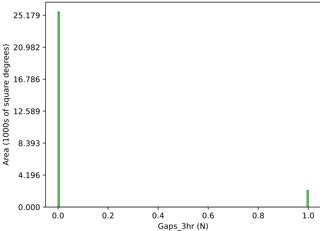
ddf_acor_sf15_lsf20_lsr50_v3.4_10yrs g band: Gaps_3hr
